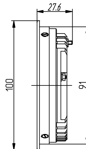
Outline drawing (in mm)
