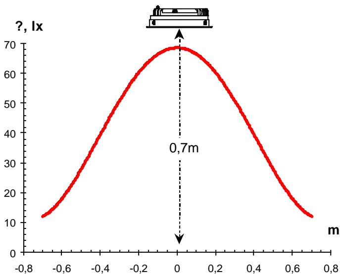
Distribution of illuminance
