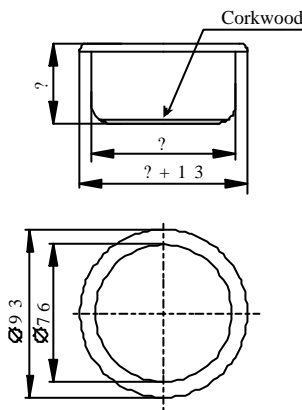
Glass-holder P/N 325881.002
