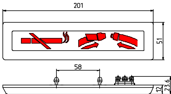
Sign «No Smoking and Fasten Seat Belt» P/N 336303.001
