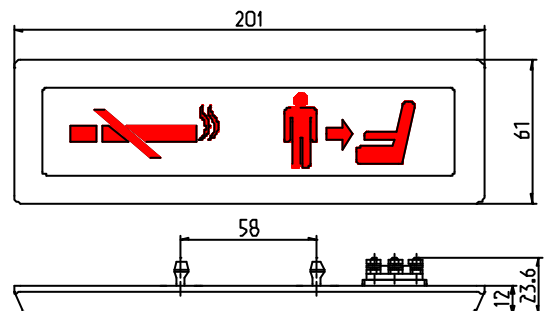
Sign «No Smoking and Return To Seat» P/N 336303.002
