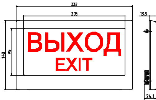
Exit sign ES-2 P/N 335101.001
