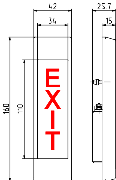
Exit sign ES-3 P/N 335101.003
